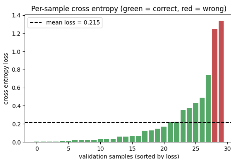
Figure 3: Per-sample cross-entropy loss on the validation set, sorted from lowest to highest. Correctly classified samples are shown in green, misclassified samples in red.
